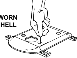
Removing a Worn Plate Roller Shell
